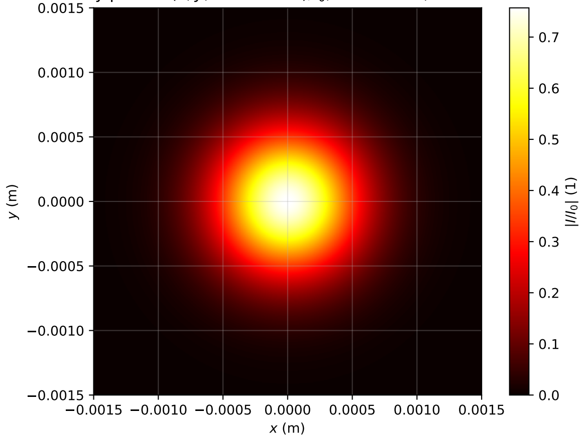
Intensity profile I(x, y, z = 1.433m)/I_0 , P_{in}=0.2P_{cr} , artificial time
